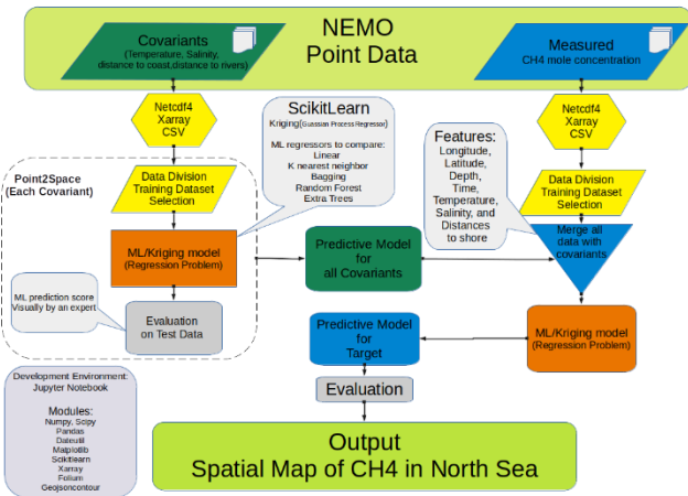
Figure 1: Flowchart for the point to space problem example using the NEMO oceanographic data.
